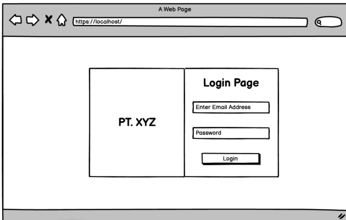
Gambar 2: Mockup Login
